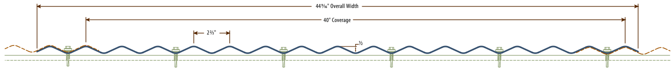
Cor-Pan 0.5 Profile
