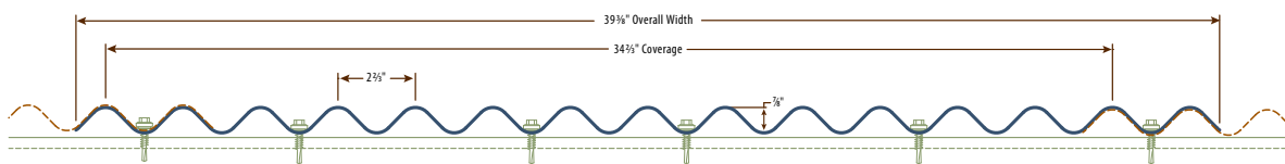
Cor-Pan 1.0 Profile
