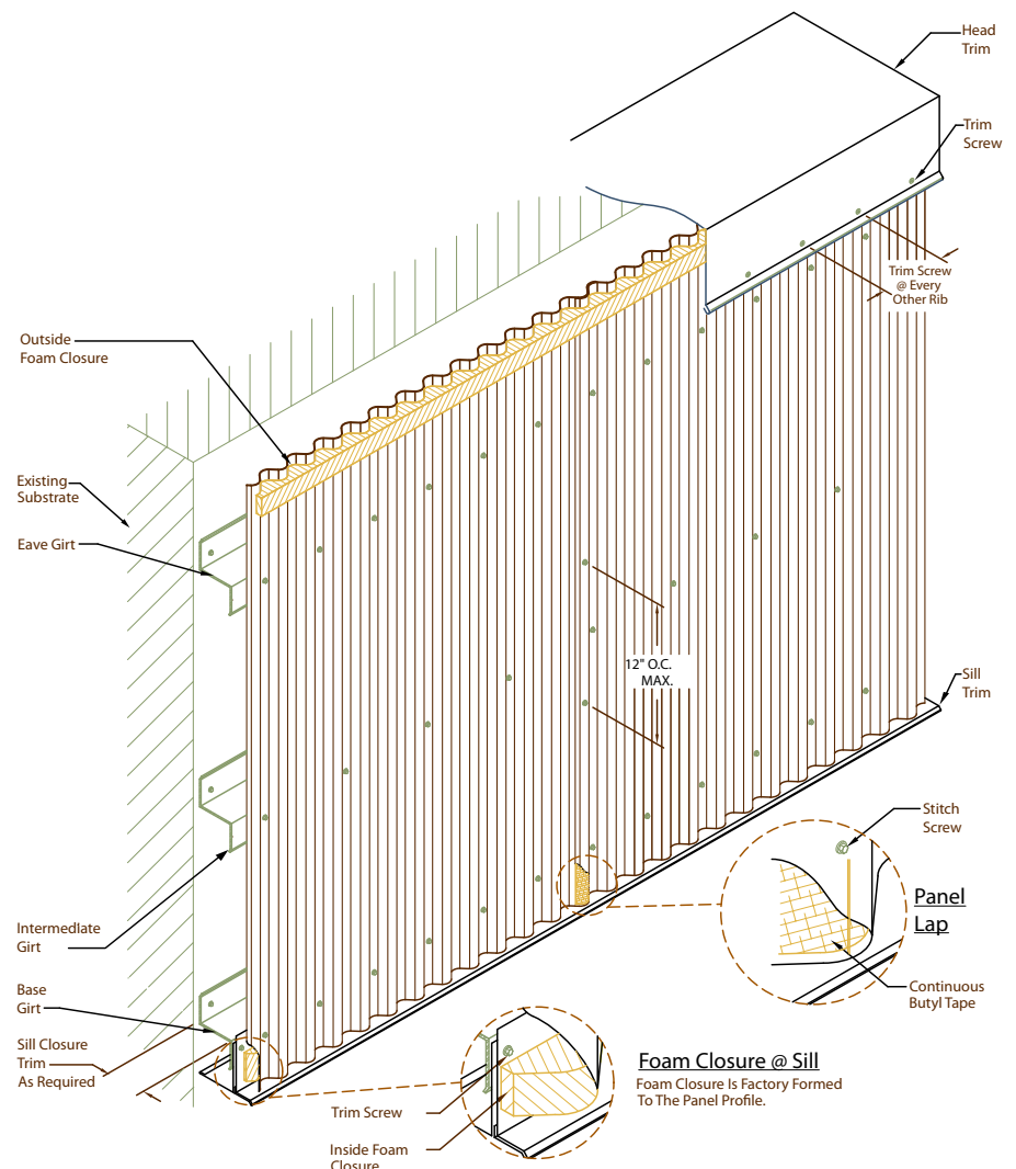
Cor-Pan 1.0 Profile
