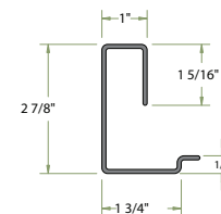
Gable Clip 18 Ga. Galv. Steel 18 Ga. Stainless Steel
